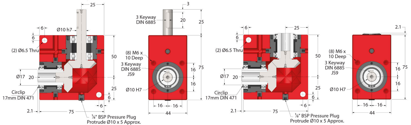
BLHI40 (Bore Input) & BLHO40 (Bore Output) Type 1:1 ratio BLHI40 only
