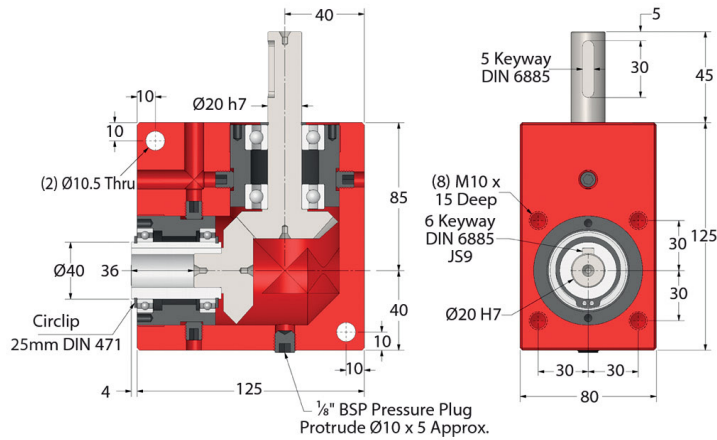
BLHI60 (Bore Input) & BLHO60 (Bore Output) Type 1:1 ratio BLHI60 only
