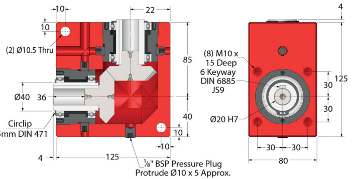
BLHB60 Type (Bore Input & Bore Output)
